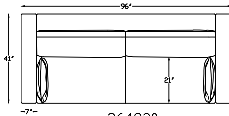
264820 TWO ARM SOFA
